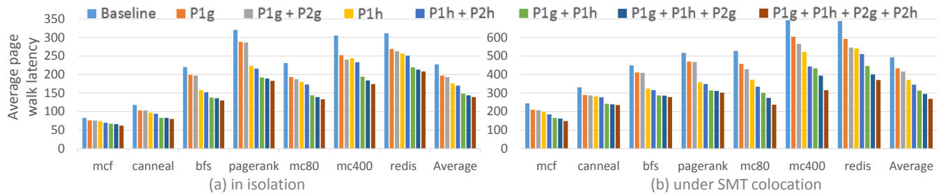
Figure 10: Average page walk latency with virtualization (a) in isolation, (b) under SMT collocation. Lower is better. Note the different scaling of y-axis between the subfigures.
