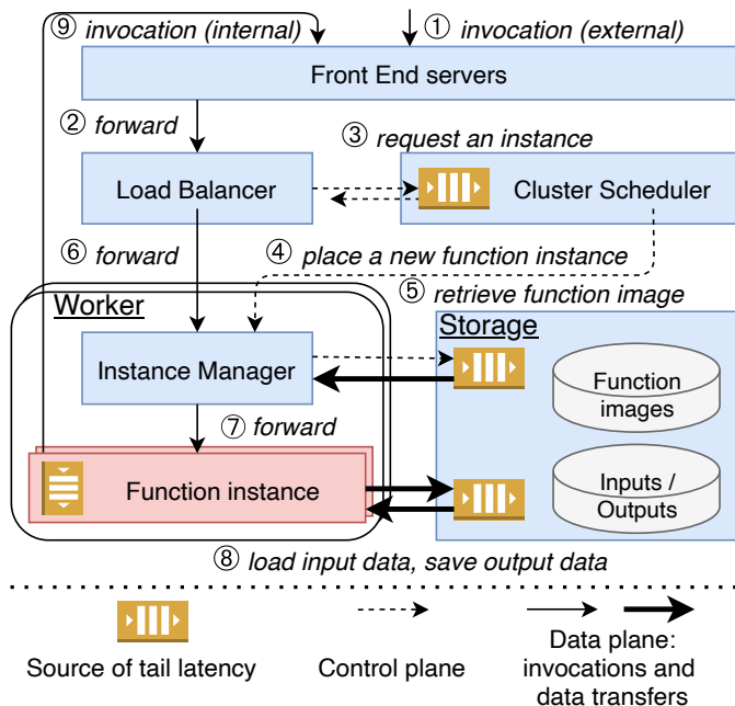
Figure 1: Serverless infrastructure overview.
